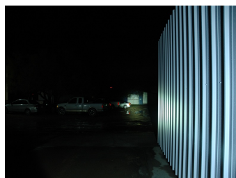
This photo shows the BBLG-LEDBLT-24V-HGL in spot configuration. The building in the distance is 300' away, well illuminated by the LED spotlight.
